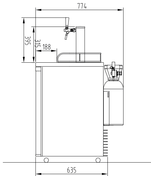
Side Elevation With CO2 Cylinder Mounted
