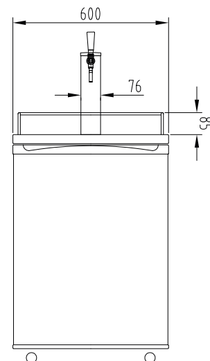
Front Elevation
