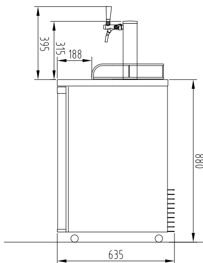
Side Elevation Without CO2 Cylinder Mounted
